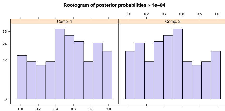
Figure 3: plot(m2)
